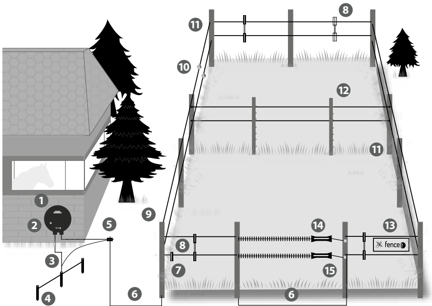
Figure No. 6: Wiring of electric fencer
